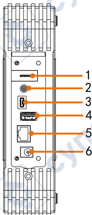
Figure 3-2 Rear Panel
