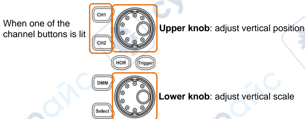
Figure 3-10 Vertical Control
