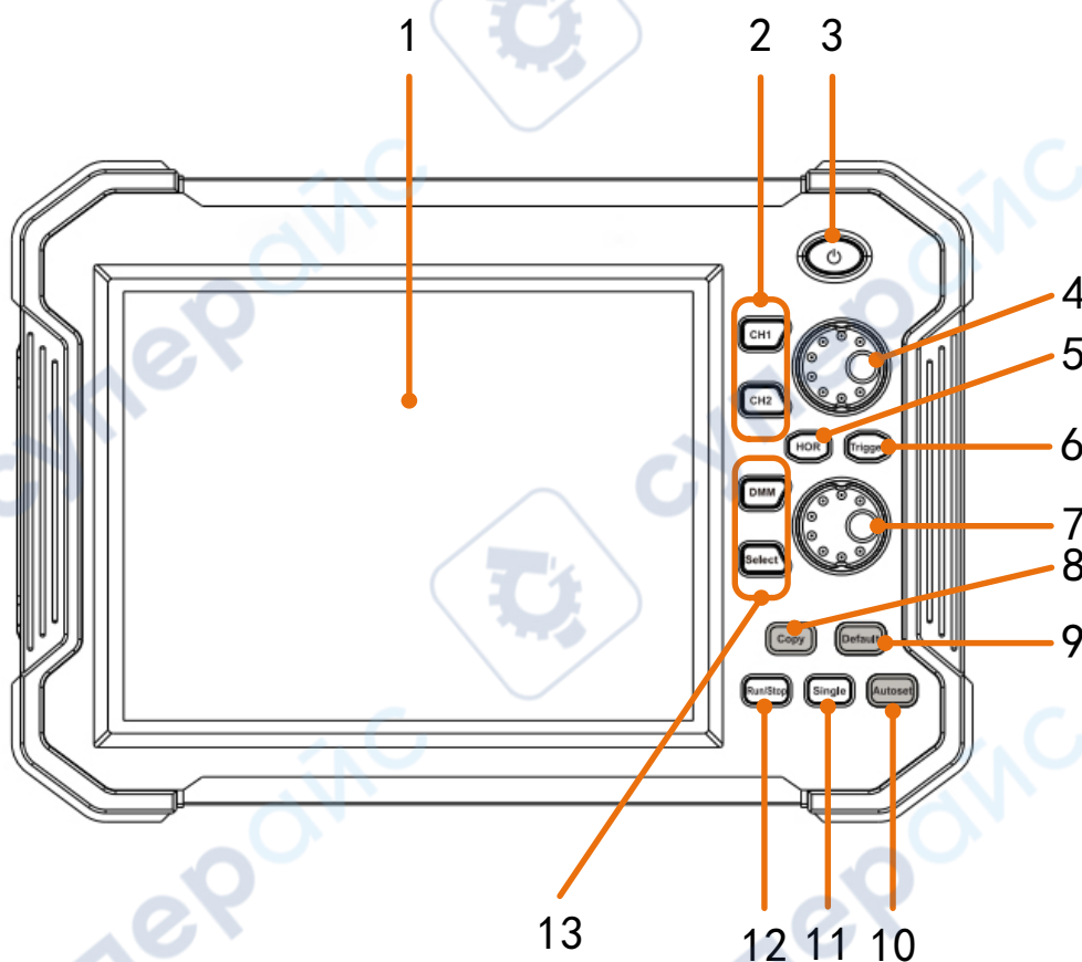
Figure 3-1 Front panel
